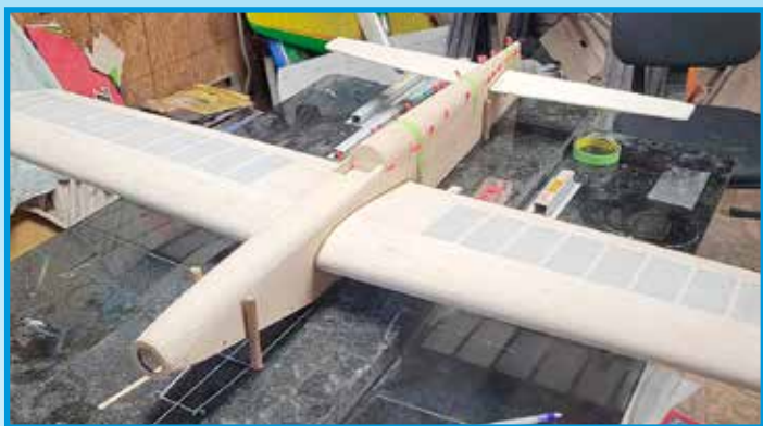
This is my plane in a Jig that I made at my job. It is a piece of granite, machined by a CNC to keep my fuselage strait during building, and for aligning the wing and stabilizer.
