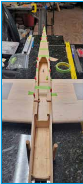
Balsa bottom block being glued on, after pipe floor installation.
